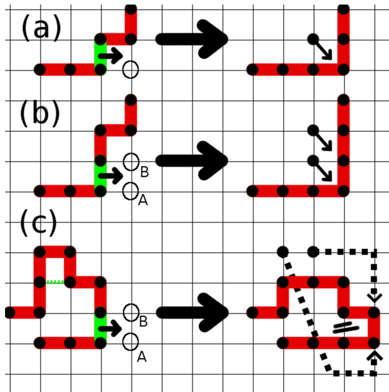
Figure 4. Implementation of pull moves for a SAP. A bond (green) is randomly selected, and in one of the randomly chosen directions perpendicular to the bond (indicated by small black arrows on the green bond) the nearest two lattice sites in this direction are randomly labelled A and B. The pull move then proceeds as follows. The vertex next to the site B is moved onto A. This can result in three cases: (a) The next vertex in the sequence of the walk lies on B, in which case the move is a bond flip. (b) The next-to next vertex in the sequence is adjacent to B, in which case a double bond flip is performed by moving the vertex in between onto B. (c) Otherwise the SAP is traverse until a kink is encountered. The kink is removed and inserted on A and B. When the resulting object is not a SAP, the move is defined to leave the state unchanged.
