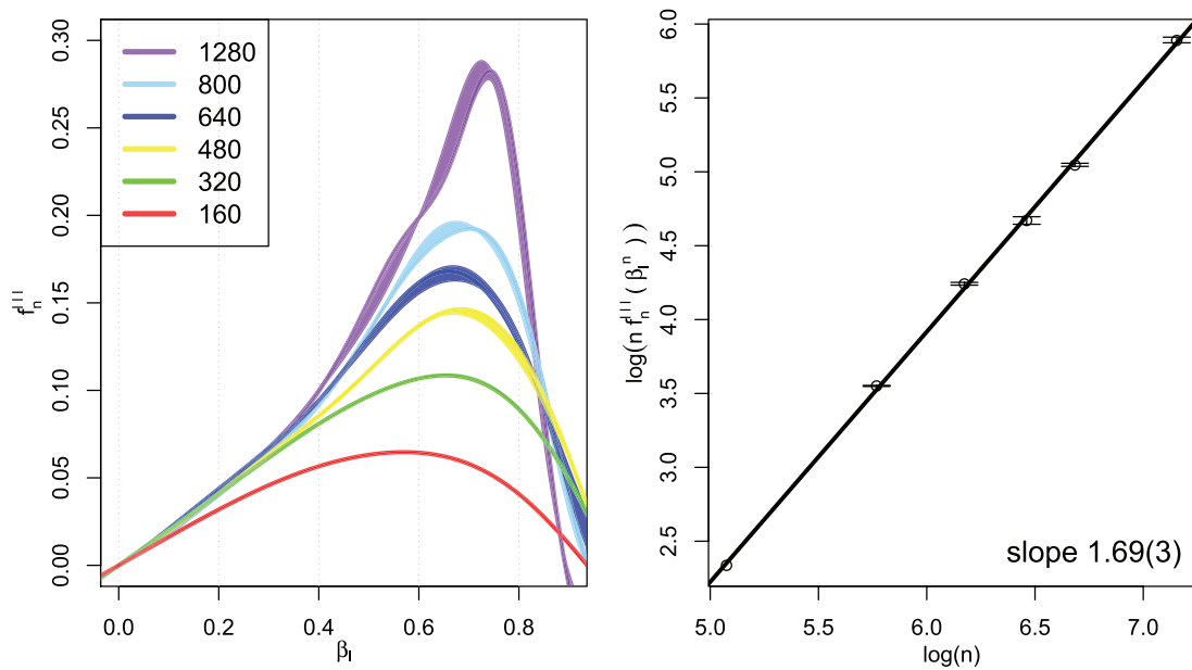
Figure 8. Left graph: scaling of the third derivative of the free energy with respect to \beta_l at \beta_h = 2.5 . Right graph: values of the maximum in n f'''_n(\beta_h = 2.5) against the length in log-log-scale, together with a linear fit indicating a slope of 1.69(3).
