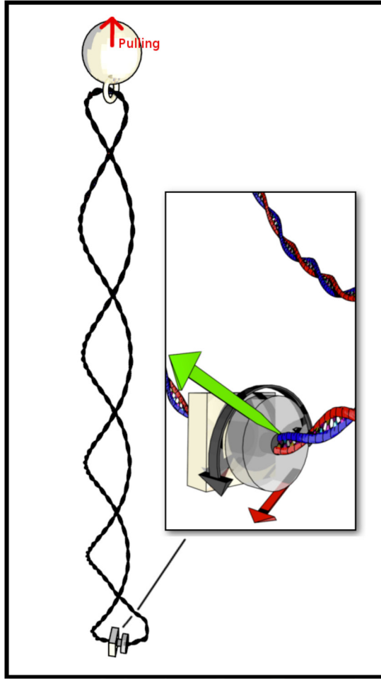
Figure 1. Sketch of the thought experiment. Both sides of a DNA like polymer are attached to the apparatus via a bead that can be acted upon with a magnetic tweezer, and a cylinder. The depicted cylinder can be rotated (black arrows). The twist-storing polymer exerts a force f on the cylinder which attacks at a distance r from the centre (green arrow). On the other hand, a force F (red arrow) can be applied at a distance R from the centre. Then, the net torque exerted on the cylinder reads FR - fr .
