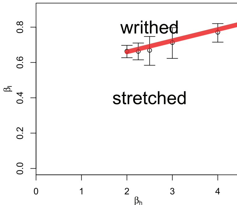
Figure 9. Phase diagram in the force-torque plane. The red line marks a second-order phase transition. We cannot properly determine the position of the transition for small pulling forces.
