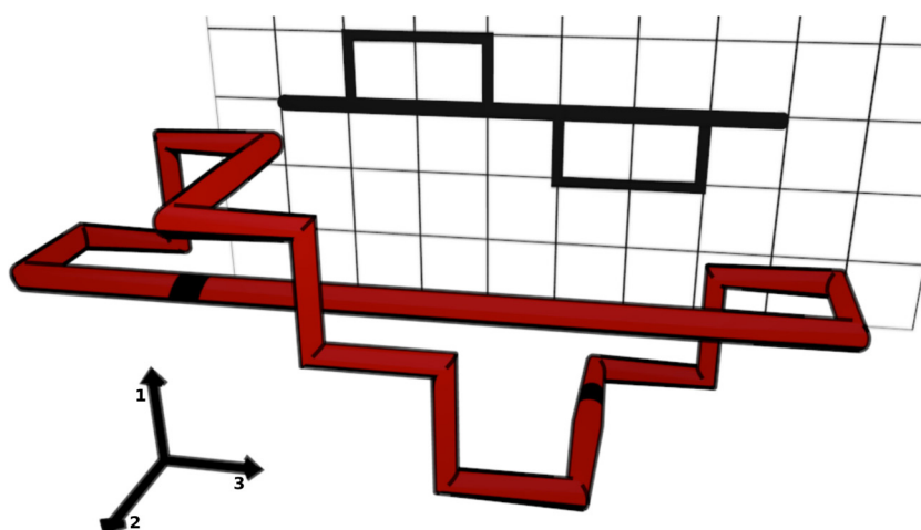
Figure 3. Directed SAUK with axis of length 24.
