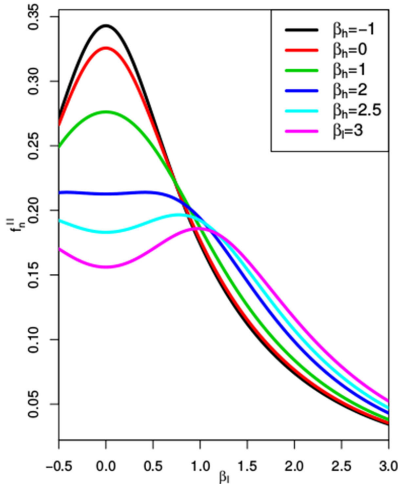
Figure 6. The figure shows the writhe fluctuations per length at selected pulling forces \beta_h against the torque \beta_l for length n = 80 .
