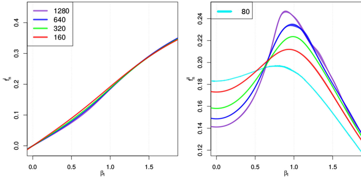
Figure 7. Scaling of the estimates of the first and second derivative of the free energy f_n with respect to \beta_l against \beta_l at \beta_h = 2.5 .
