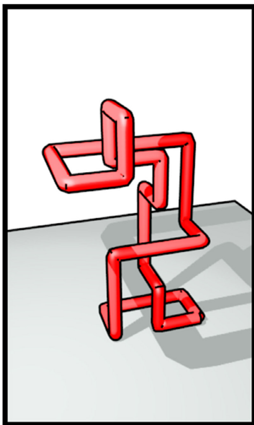
Figure 2. A self-avoiding unknot (SAUK) above a surface of length n = 28 . The step furthest away from the surface defines the extension h .
