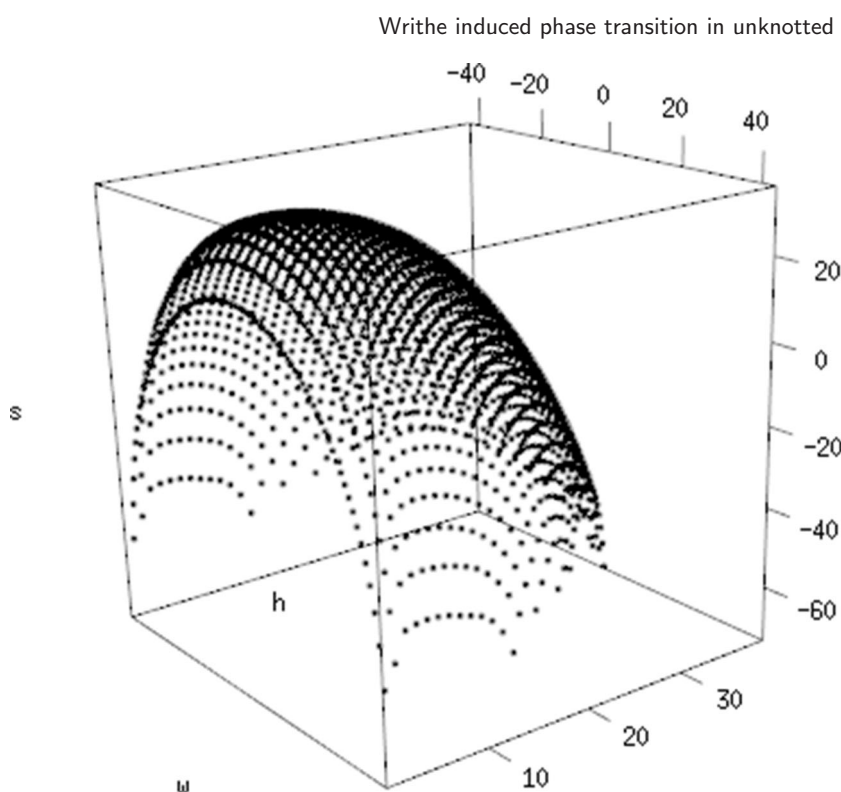
Figure 5. Two-dimensional entropy s of the self-avoiding unknot at n = 80 over the extension h and the writhe w = 4Wr . This entropy lacks macrostates w > 42 as well as the macro state (w = 0, h = 0) . The problem of generating samples of planar polygons in three dimensions with the pull moves has been addressed in the appendix of [38].
