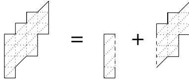
Figure 2. The decomposition of a four-column parallelogram polyomino into its first column and remainder; the dashed edges are internal edges of the polyomino.
