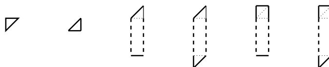
Figure 10. Types of possible single-column parallelogram polyominoes.
