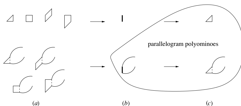
Figure 7. Obtaining an expression for \hat{P}(x, y, d) : (a) Parallelogram polyominoes with right height of 1; (b) the set of lattice objects with perimeter generating function T_1(x, y, d) ; (c) parallelogram polyominoes with left height of 0; the ringed objects are then all the parallelogram polyominoes.
