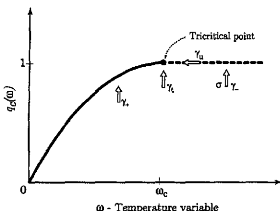
Figure 1. The radius of convergence, q_c(\omega) , of \mathcal{G}(q, \omega) in the IPDSAW model, showing the tricritical point at (\omega_c, 1) . For other models the right-hand side of the curve need not run along q = 1 . The arrows indicate the paths on which the various exponents are defined.
