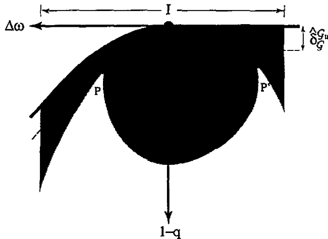
Figure 4. A schematic illustration of the region that is contained in the \varepsilon -asymptotic region \Delta_G^u . The wings are the regions bounded by the y_3 line (and its \omega \geq \omega_c counterpart), while the middle is the scaling region defined by the locus of values \delta_G^u(y) which are strictly positive for y \in [0, y_3] . The intersection of these two regions defines the point P (and for \omega \geq \omega_c the point P' ). These points are below the critical line by construction and so allow us to choose the uniform value \hat{\delta}_G^u . The region defined by the \hat{\delta}_G^u curve and the critical line is then certainly contained in \Delta_G^u .
