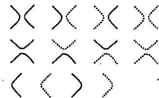
Figure 7. Allowed vertices for the two-colour loop model. Colours 1 and 2 are indicated by full and broken curves, respectively. The Boltzmann weights are, respectively, \sin(\lambda - u) , \sin u and 1 for vertices in the three rows.
