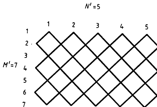
Figure 1. A 7 \times 5 lattice of the rotated orientation.
