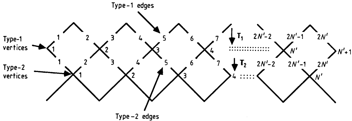
Figure 3. Examples of the two different types of rows of vertices and edges that occur in this model. A T_1 ( T_2 ) transfer matrix acts on a type-1 (2) row of edges to add a type-2 (1) row of edges. In doing so it creates a type-1 (2) row of vertices.
